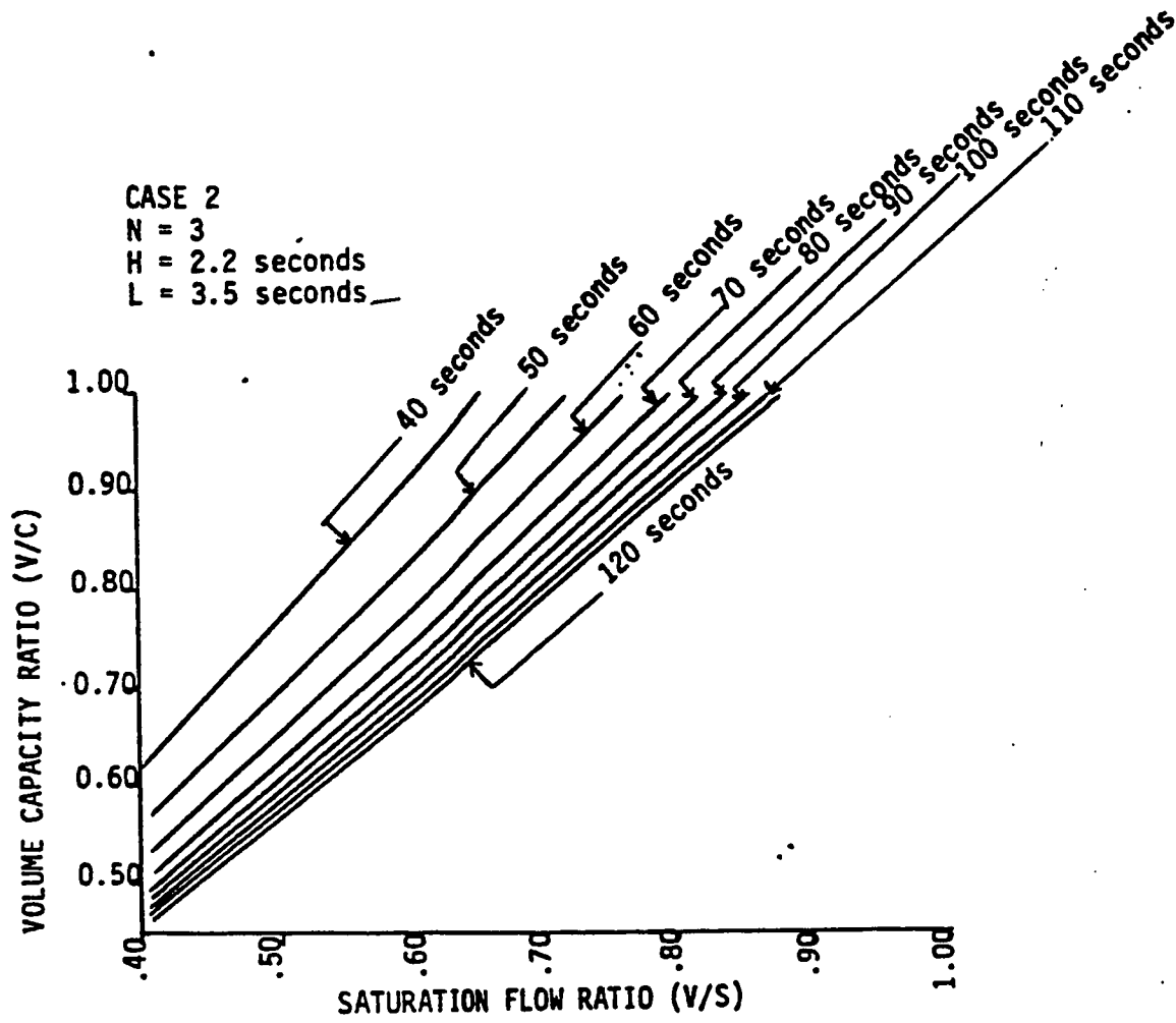
Figure 3.5. Relationship between V/S & V/C
