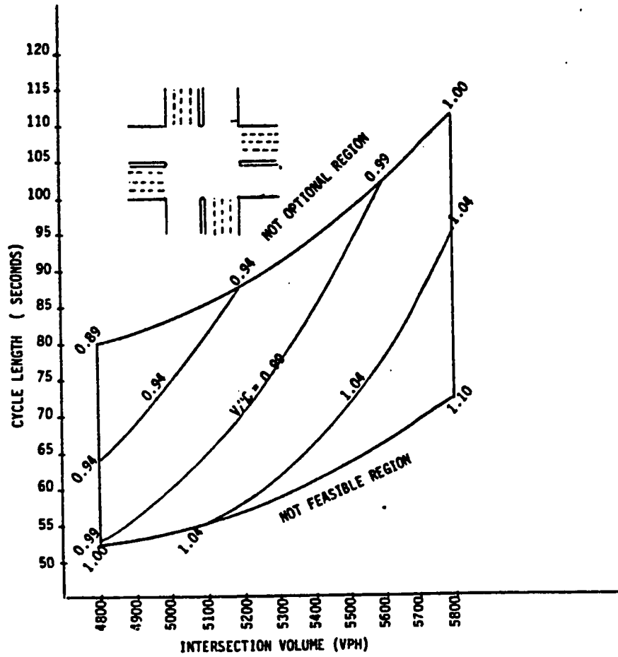
FIGURE 3.12. NOMOGRAPH FOR OPTIMUM CYCLE LENGTH (seconds)
