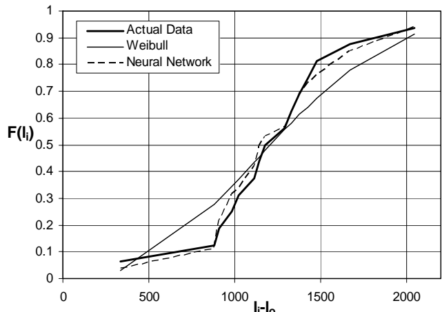
Figure 11(d). Failure rate F(i) for Boeing 737 brake assembly B_4 versus failure data (landings) using number of landings parameter
