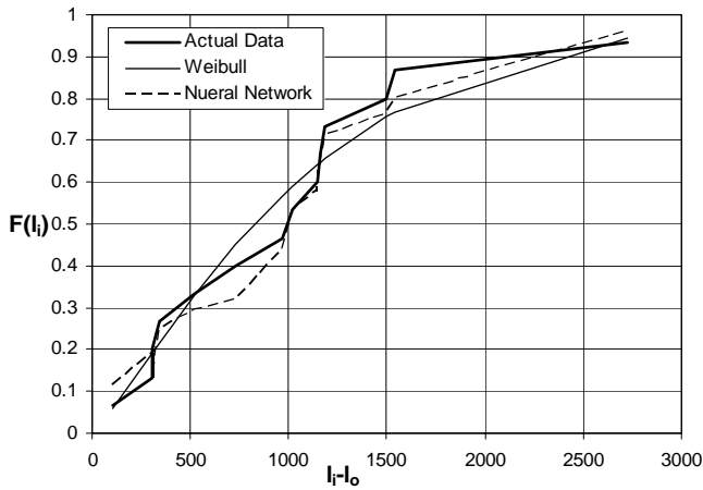
Figure 11(a). Failure rate F(i) for Boeing 737 brake assembly B_1 versus failure data (landings) using number of landings parameter
