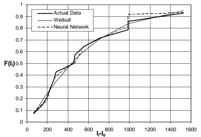
Figure 11(b). Failure rate F(i) for Boeing 737 brake assembly B_2 versus failure data (landings) using number of landings parameter
