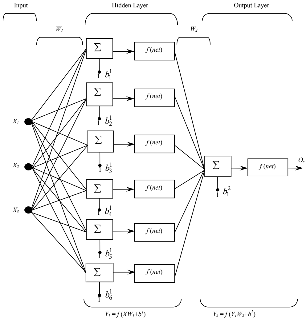
Figure 8. ANN architecture
