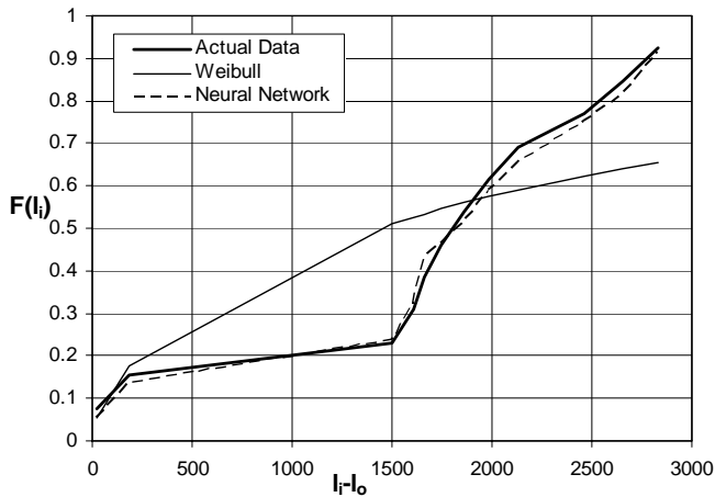
Figure 11(c). Failure rate F(i) for Boeing 737 brake assembly B_3 versus failure data (landings) using number of landings parameter
