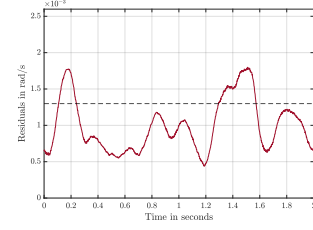
(f) Fault group 2 - Severity level 3 (F2/SV3) residuals
