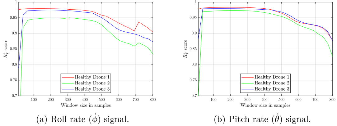
Figure 5.5: Effect of different window sizes on the differentiation of roll rate ( \dot{\phi} ) and pitch rate ( \dot{\theta} ) signals. A window size of 100 samples was found to provide a balance between noise suppression and signal fidelity. Smaller window sizes resulted in excessive noise amplification, while larger window sizes introduced over-smoothing, distorting the system's response.
