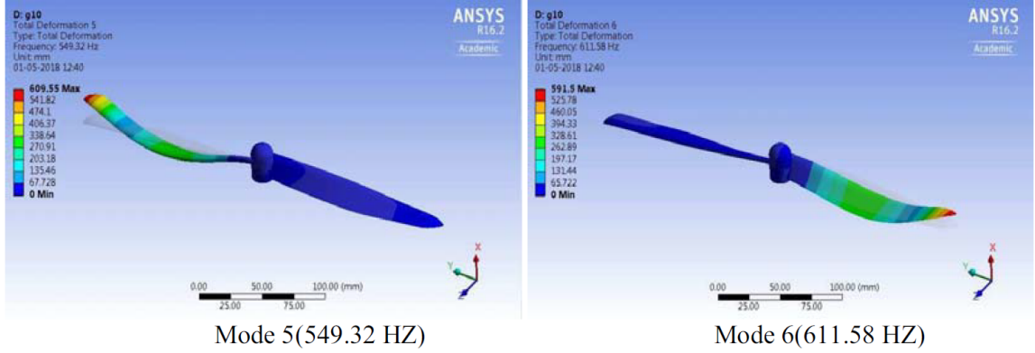
Figure 3.4: Finite Element Analysis (FEA) illustrating propeller deformation under vibrational loading. High-frequency oscillations contribute to stress accumulation, leading to crack formation and propagation [68].
