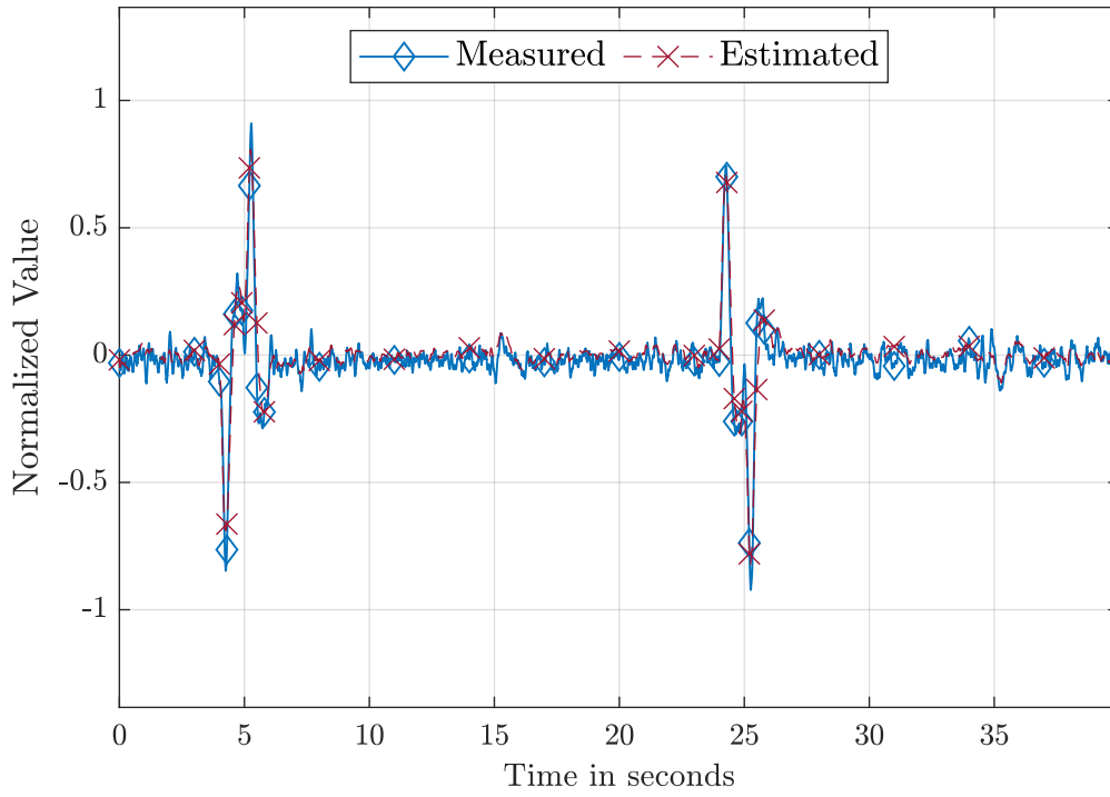
(a) Model fitting for roll rate \dot{\phi} .
