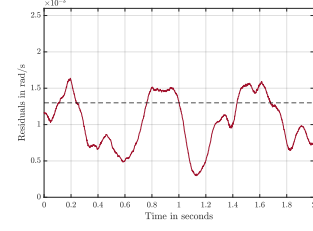
(c) Fault group 1 - Severity level 3 (F1/SV3) residuals
