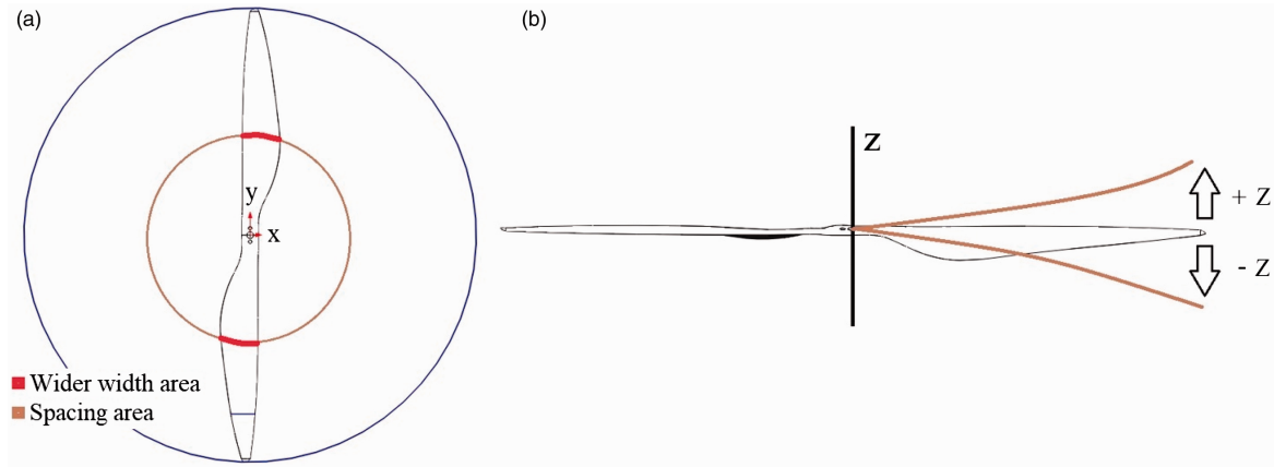
Figure 3.3: Propeller vibration induced by rotational motion. The top-down view (a) highlights regions of varying width and spacing that contribute to asymmetric aerodynamic forces, which in turn generate oscillatory motion. The side view (b) demonstrates the displacement along the z -axis, showing how the unbalance causes alternating movement in the positive and negative directions. These vibrations, if excessive, can lead to structural fatigue and crack formation [67].
