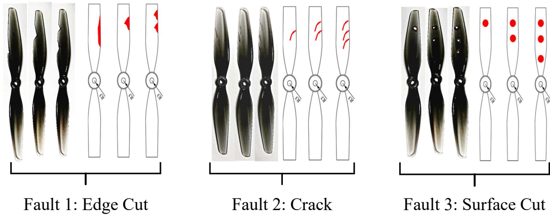
Figure 3.7: Photographs of the three fault groups for the drone propeller.
