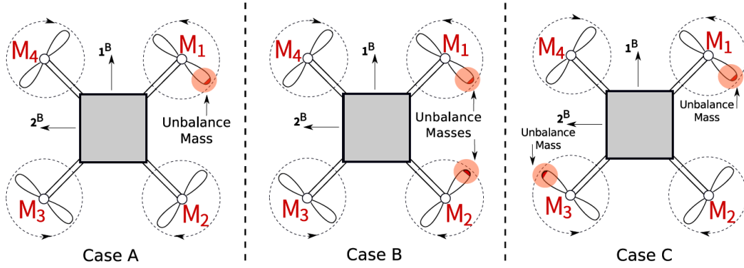
Figure 1.2: Fault combinations using different numbers and locations of defective propellers [9].
