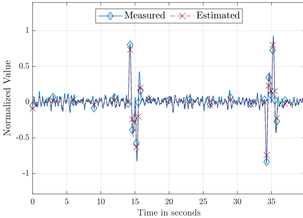
(b) Model fitting for pitch rate \dot{\theta} .
