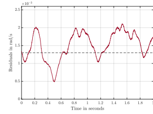
(i) Fault group 3 - Severity level 3 (F3/SV3) residuals
