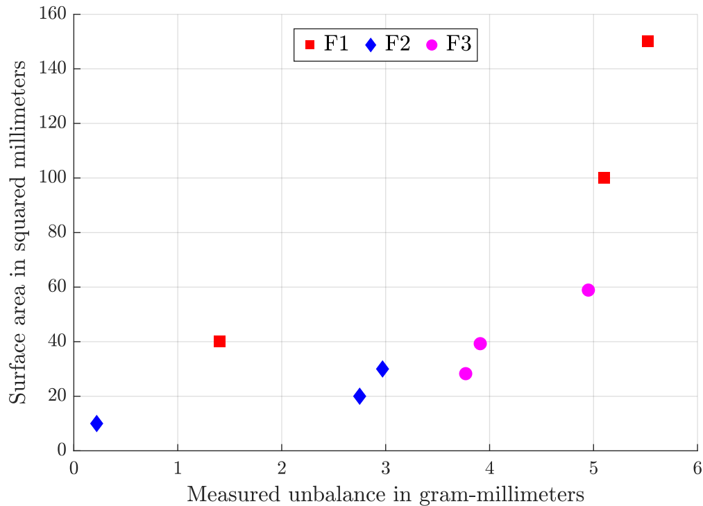
Figure 3.12: Distribution of Fault Types Based on Measured Unbalance and Surface Area
