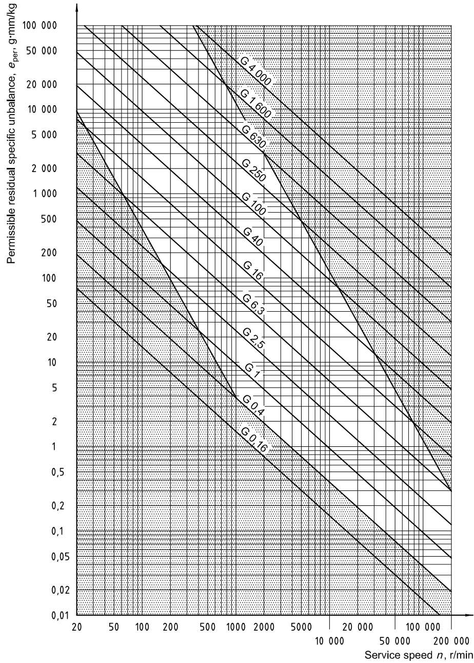
Figure 3.5: Permissible residual specific unbalance as a function of balance quality grade G and service speed n , adapted from ISO 1940-1:2003. The white area indicates the commonly used range based on industry standards.
