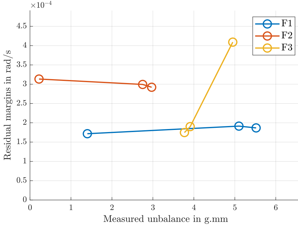
Figure 5.12: Analysis of fault severity effects across different fault types. The relationship between residual margins and measured unbalance highlights distinct severity trends for each fault category.
