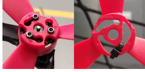
(b) Friction removal from the propeller lock [44].
