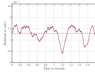
(h) Fault group 3 - Severity level 2 (F3/SV2) residuals
