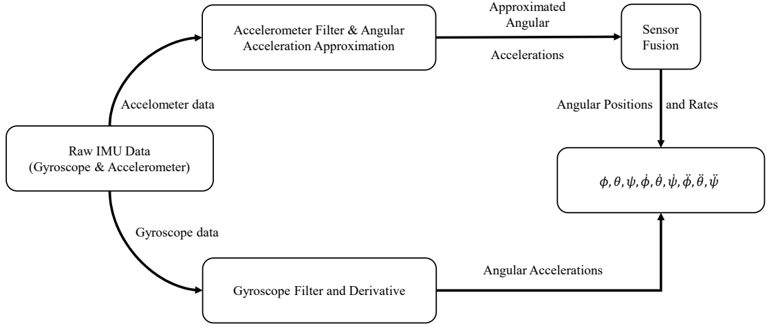
Figure 2.3: Estimation framework for converting IMU reading to the nine attitude states.
