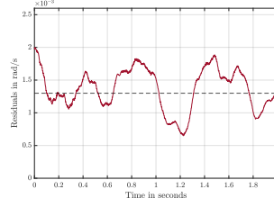
(e) Fault group 2 - Severity level 2 (F2/SV2) residuals
