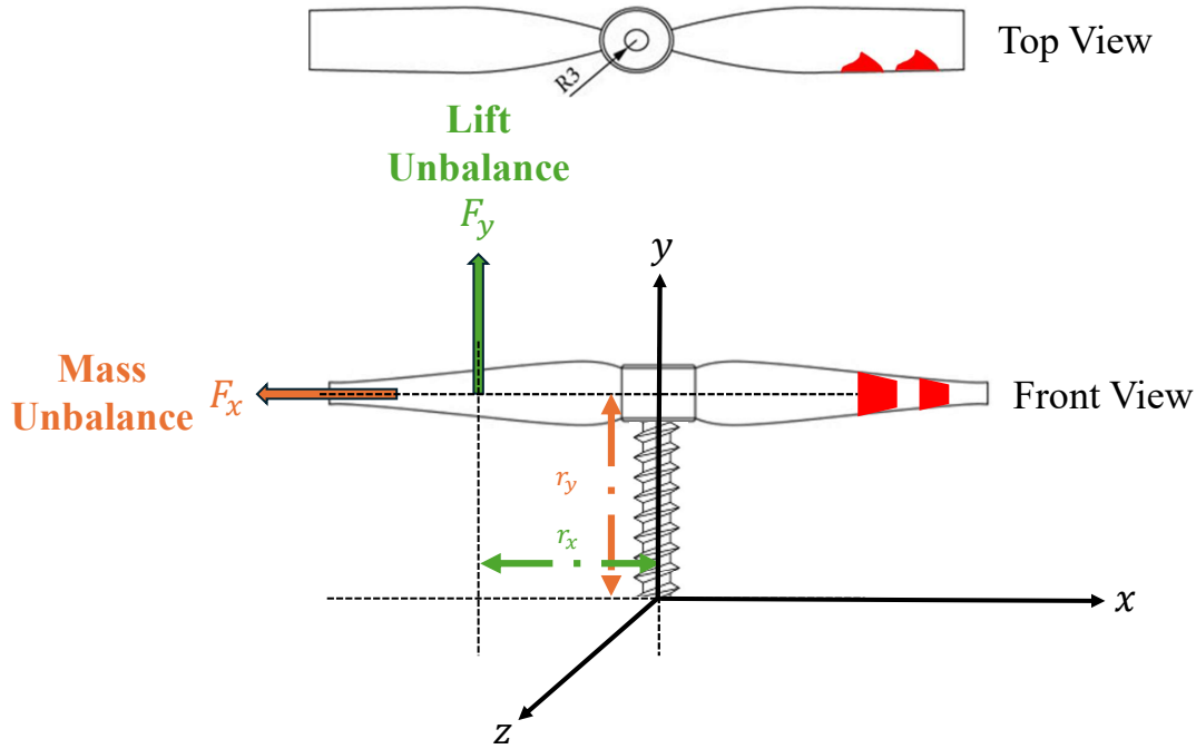
Figure 5.11: Effect of edge cuts on aerodynamic and unbalance torques. The top view illustrates material removal from the blade edges, shifting the center of lift toward the healthy blade. The front view highlights how the reduction in lift unbalance torque (clockwise) and the mass unbalance torque (counterclockwise) influence the system. Both torques scale with \Omega^2 , maintaining opposing effects.
