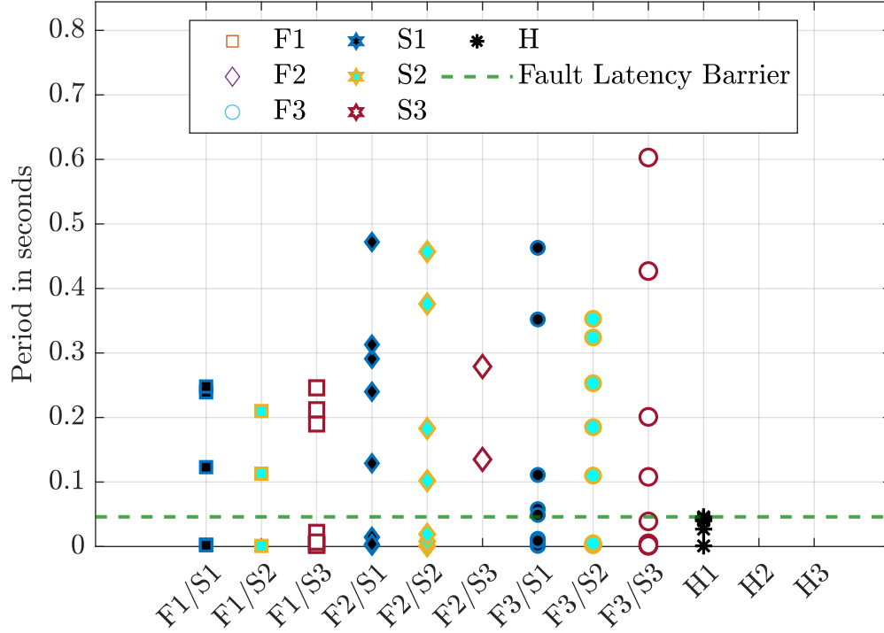
Figure 5.9: Durations of residual margin of the roll rate \dot{\phi} crossings for nine fault samples and three healthy samples (FSDs). The plot highlights the periods during which the residuals exceeded the predefined healthy margin, with fault samples showing prolonged deviations compared to healthy samples. The maximum margin crossing period of the healthy samples is used to define the FML threshold.
