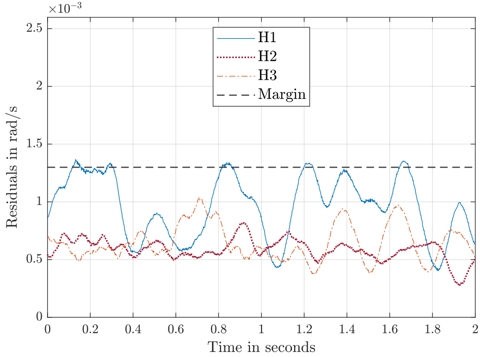
(a) Residuals of the roll rate model G_{\dot{\phi}} across three healthy drones.
