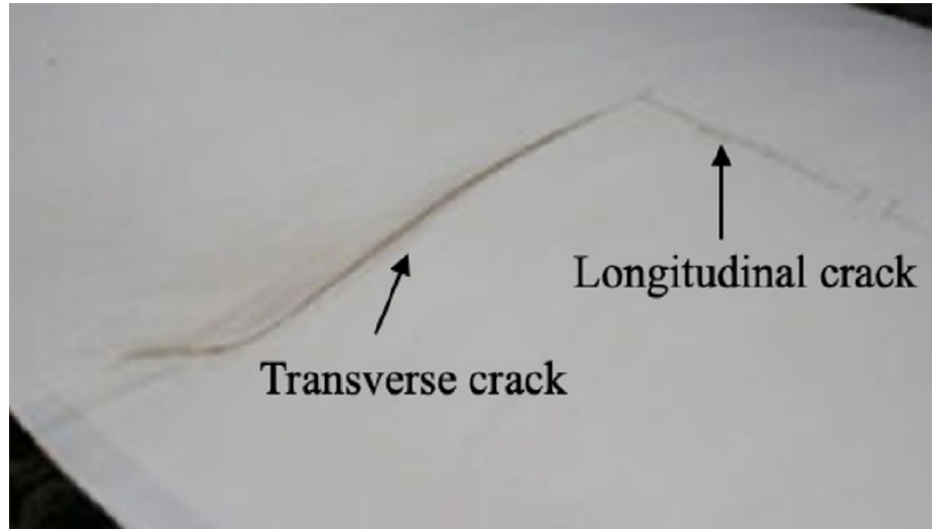
Figure 3.2: Crack types on propeller blades (Transverse & Longitudinal) [64].
