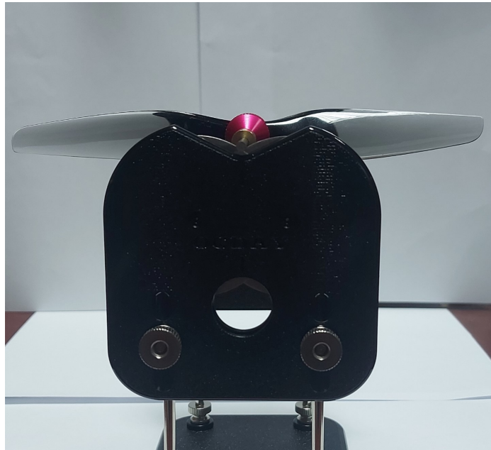
Figure 3.9: A properly balanced propeller remains stationary at any orientation on the Hobby Fans Tru-Spin propeller balancer, indicating minimal residual mass asymmetry.
