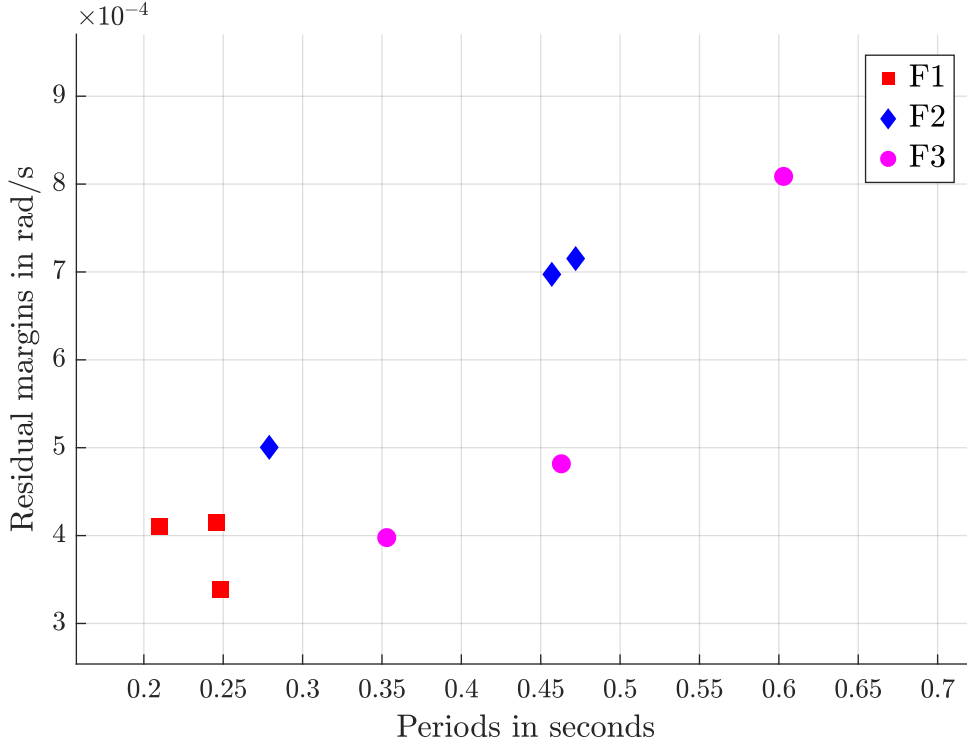
Figure 5.10: Maximum residual margin plotted against the maximum fault periods for each fault type. The plot demonstrates clear separation between fault types, enabling effective classification.
