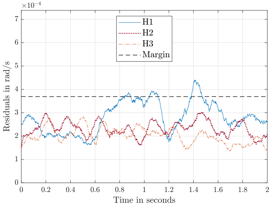
(b) Residuals of the pitch rate model G_{\dot{\theta}} across three healthy drones.
