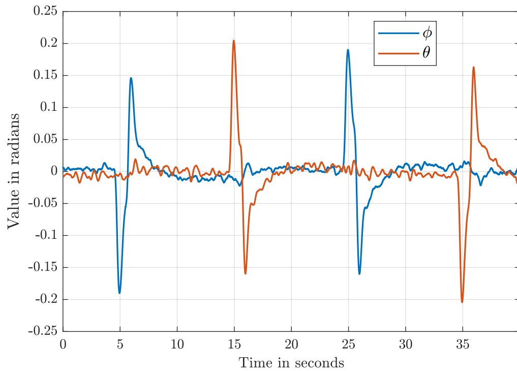
Figure 5.4: Recorded roll ( \phi ) and pitch ( \theta ) states during the square trajectory flight. Increased attitude excitations occur at trajectory corners due to rapid directional transitions.
