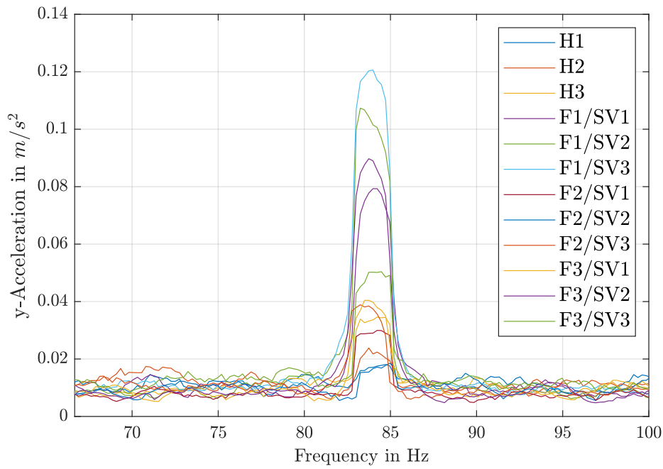
Figure 3.14: Frequency response analysis showing acceleration in the y -direction as a function of frequency for different fault conditions and severity levels. The peak at 83.3 Hz indicates the primary resonance frequency.
