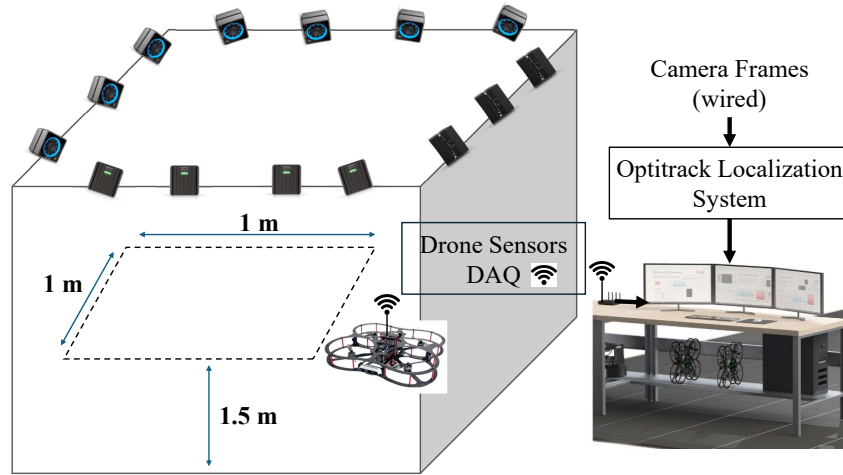
Figure 5.1: Experimental setup flow.
