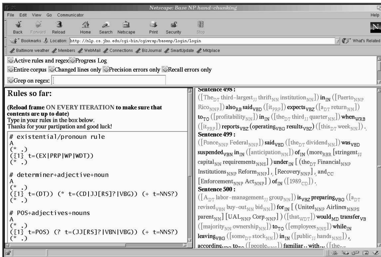
Figure 4: Screenshot of base NP chunking system
