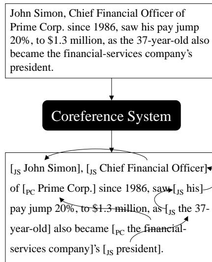
Figure 1: Coreference System
