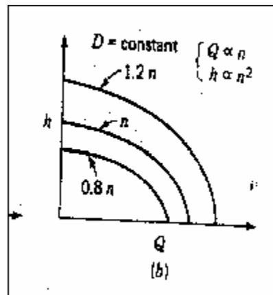
FIGURE 3 Head vs. Engine Speed (Courtesy of Fluid Mechanics, Frank M. White) The fan/pump laws requires that the motor must be able to operate a wide range of velocities, but there is a limiting factor. At standard atmospheric pressure and temperature, the velocity of sound is 1125 ft/s. As the velocity of the air reaches this speed, the airflow becomes extremely turbulent and the mechanical losses are very high. For this reason, the fan must be larger than 32 inches in diameter.
