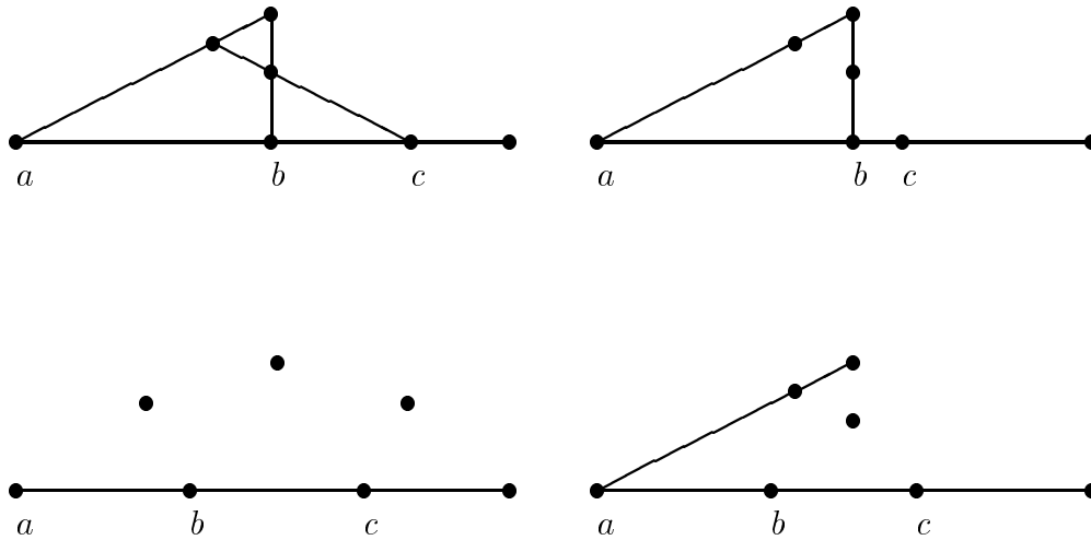
Figure 3.1. Distinguished triples in matroids with a four point line.
