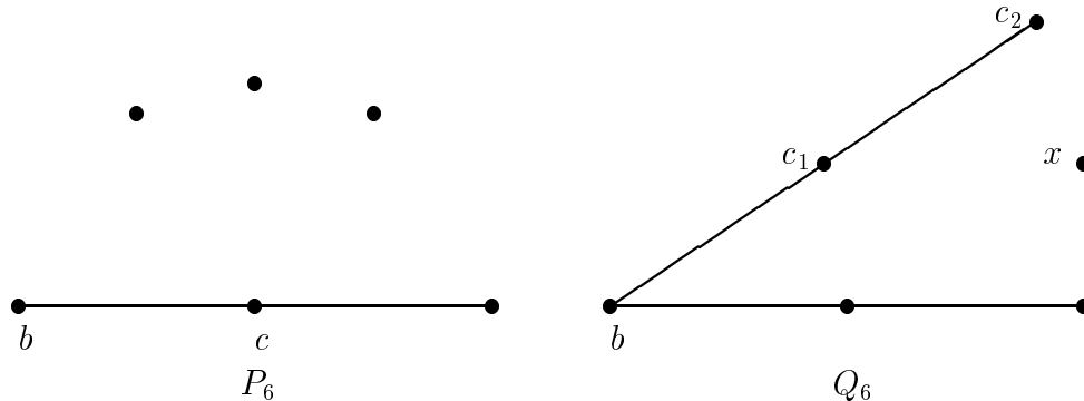
Figure 3.3 The matroids P_6 and Q_6 .
