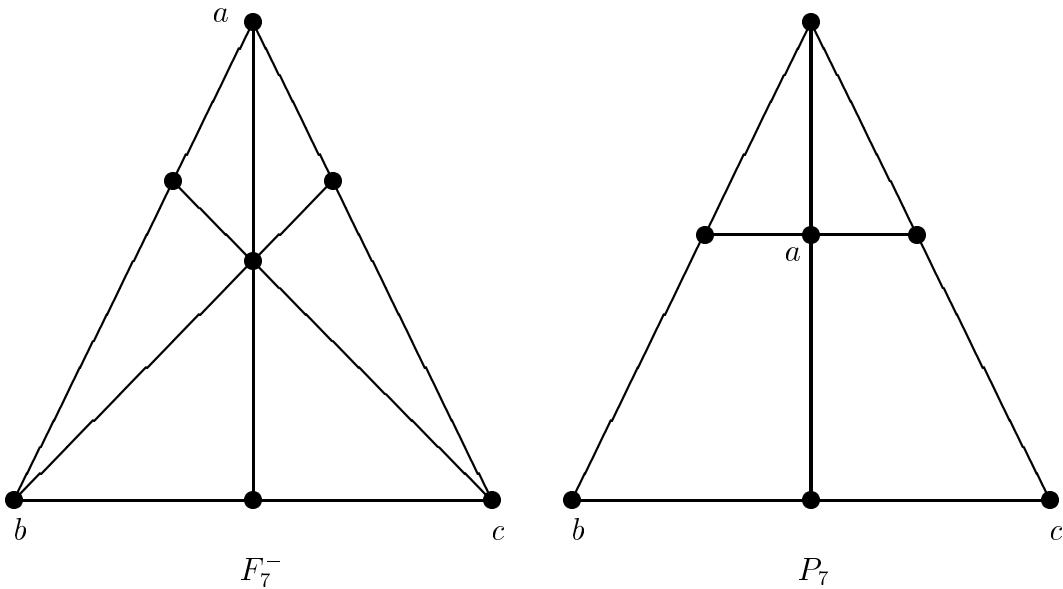
Figure 3.2. Distinguished triples in F_7^- and P_7 .
