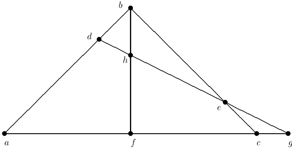
Figure 5.1 The maximum rank-3 near-regular matroid.
