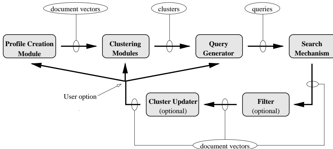
Figure 1: WebACE Architecture
