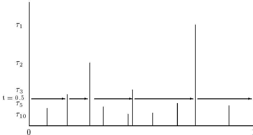
Figure 9. Kingman's coalescent
